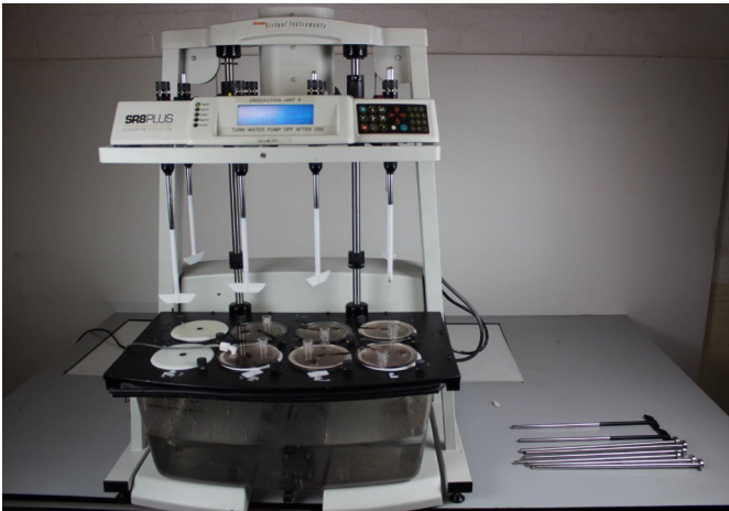
Hanson Virtual Instruments Dissolution Test Station collected from Keele
